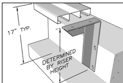
L Bracket
