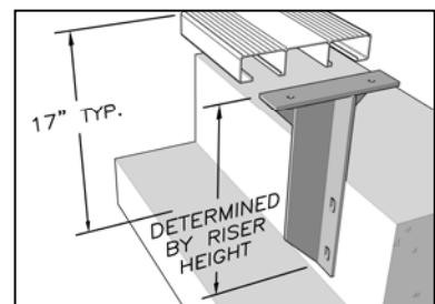
T Bracket
