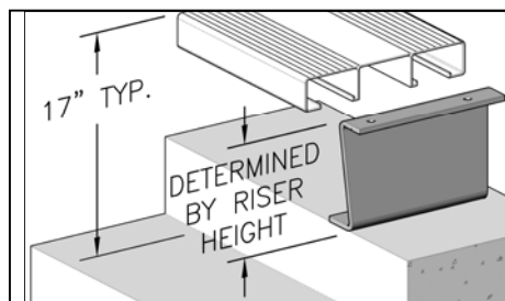
Z Bracket
